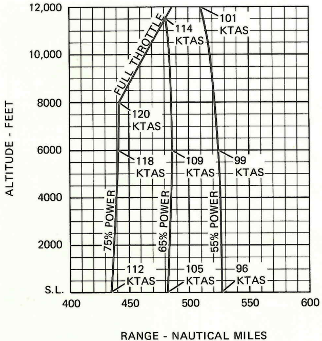
Figure 5-8. Range Profile (Sheet 1 of 3)
